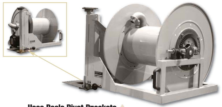
Hose Reels Pivot Brackets ▲ Bracket is attached to the side of the reel frame. The reel pivots on the bracket with positive stops at 0°, 45° and 90° locations.
